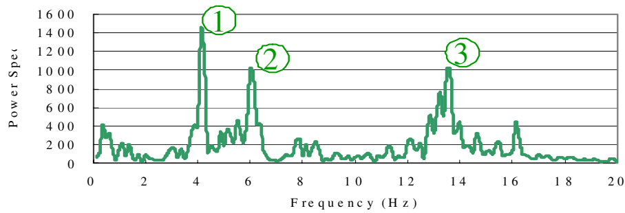
(a) PCB 393C – Mode 1: 4.12 Hz, Mode 2: 6.00 Hz, Mode 3: 13.63 Hz
