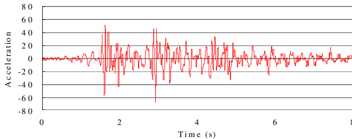
(c) Experimental results of vertical acceleration vs. time of the ADXL 202E unit.
