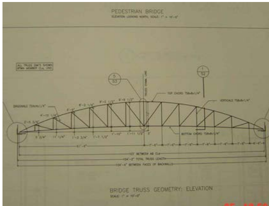
Figure 10. UC, Irvine pedestrian bridge steel truss bridge design layout provided by construction company
