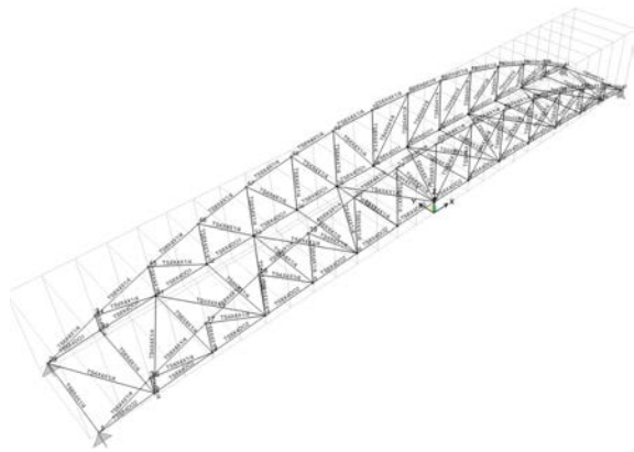
Figure 11. Three-dimensional model of bridge produced on SAP-2000 indicating all member properties and support conditions.
